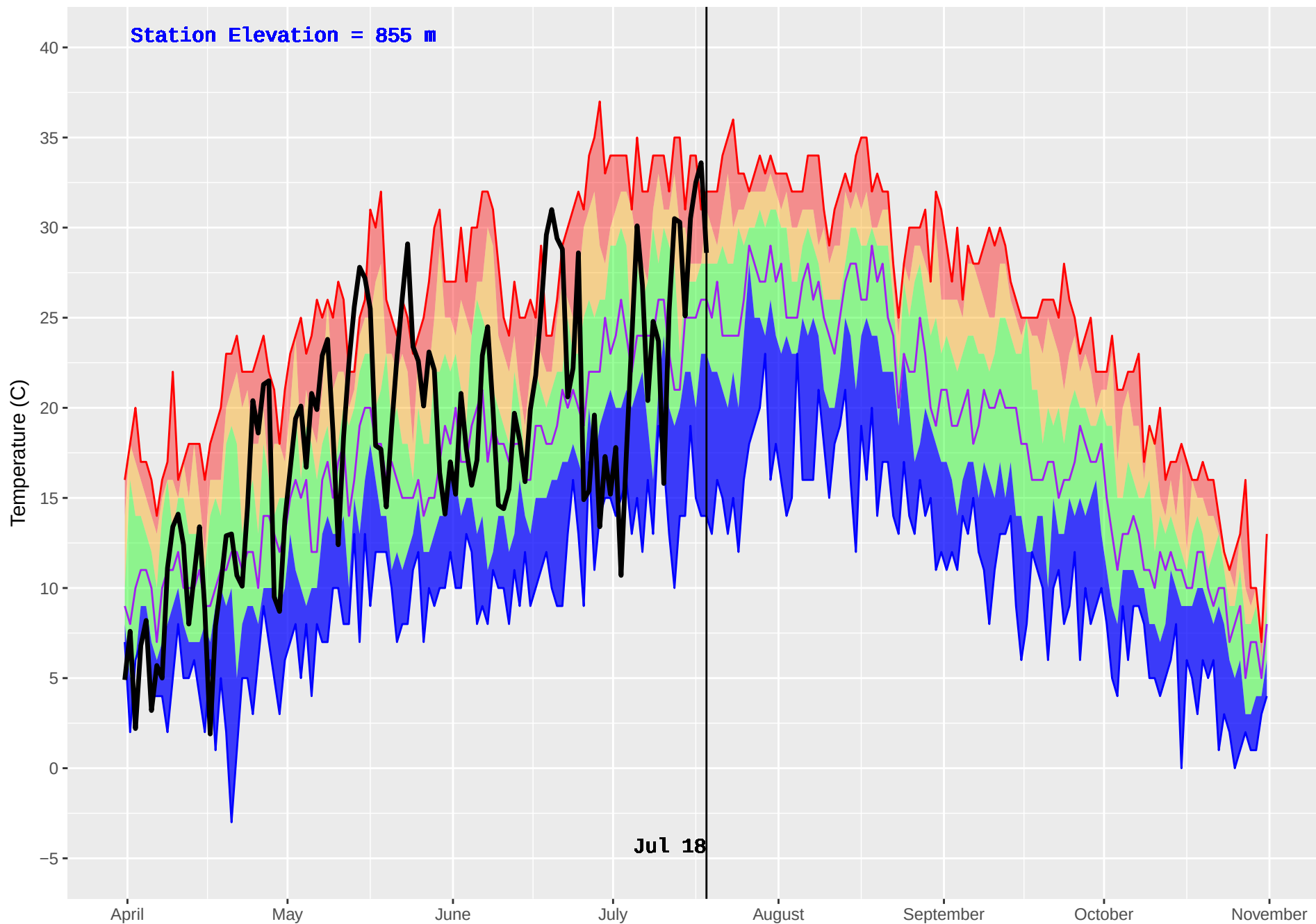
AUGUST LAKE (836) : Historical (2003–2016) and Current (2018) Daily Temperature
