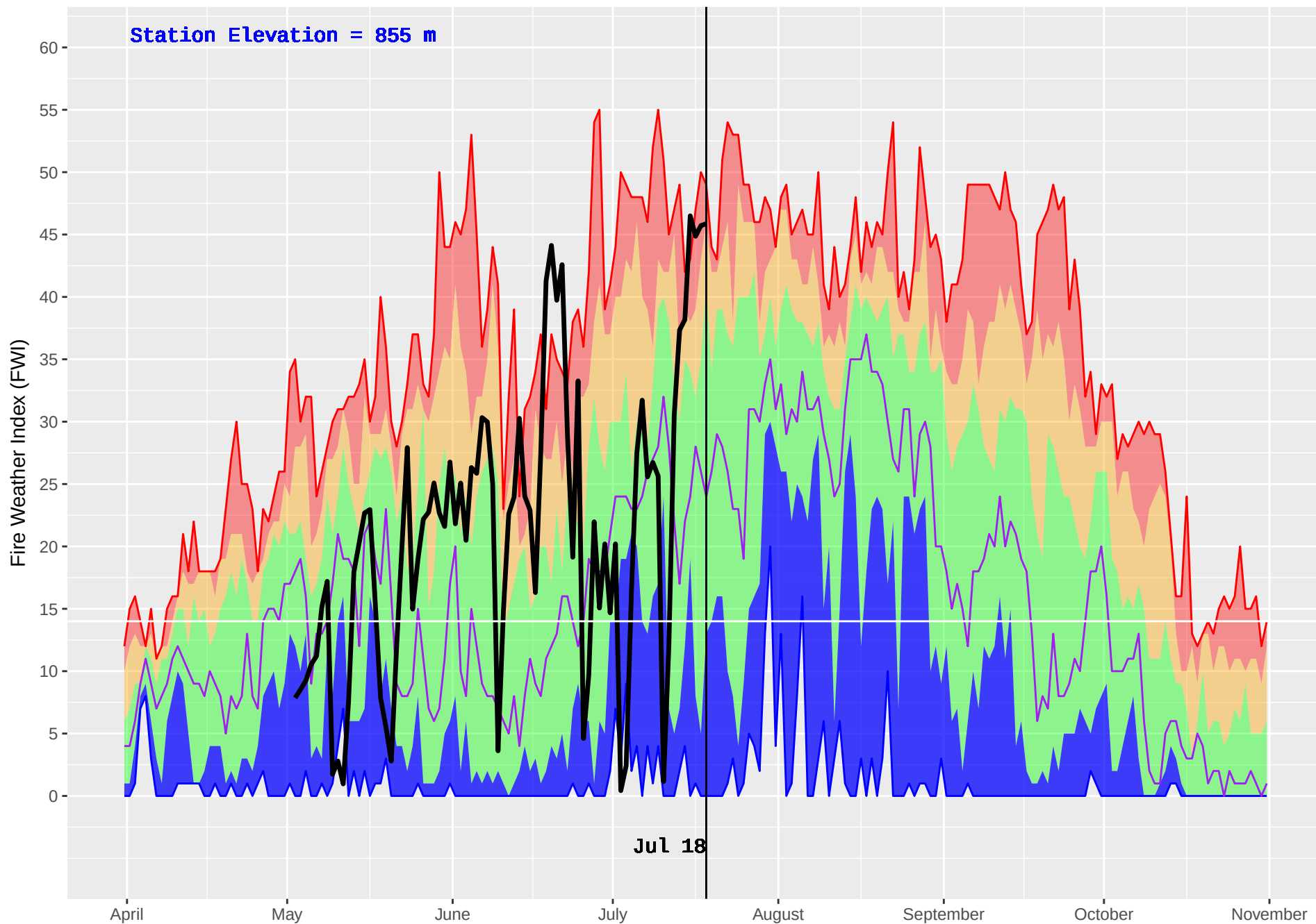
AUGUST LAKE (836) : Historical (2003–2016) and Current (2018) Daily Fire Weather Index (FWI)
